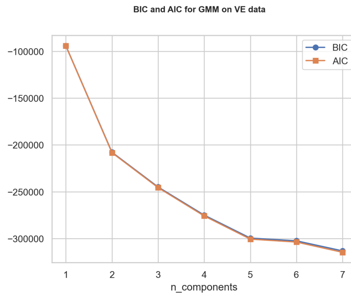
Figure 9: Comparative analysis using BIC and AIC criteria - VE perspective
